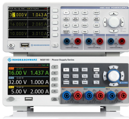
R&S®HMC8043 and R&S®NGE103B three-channel power supplies
